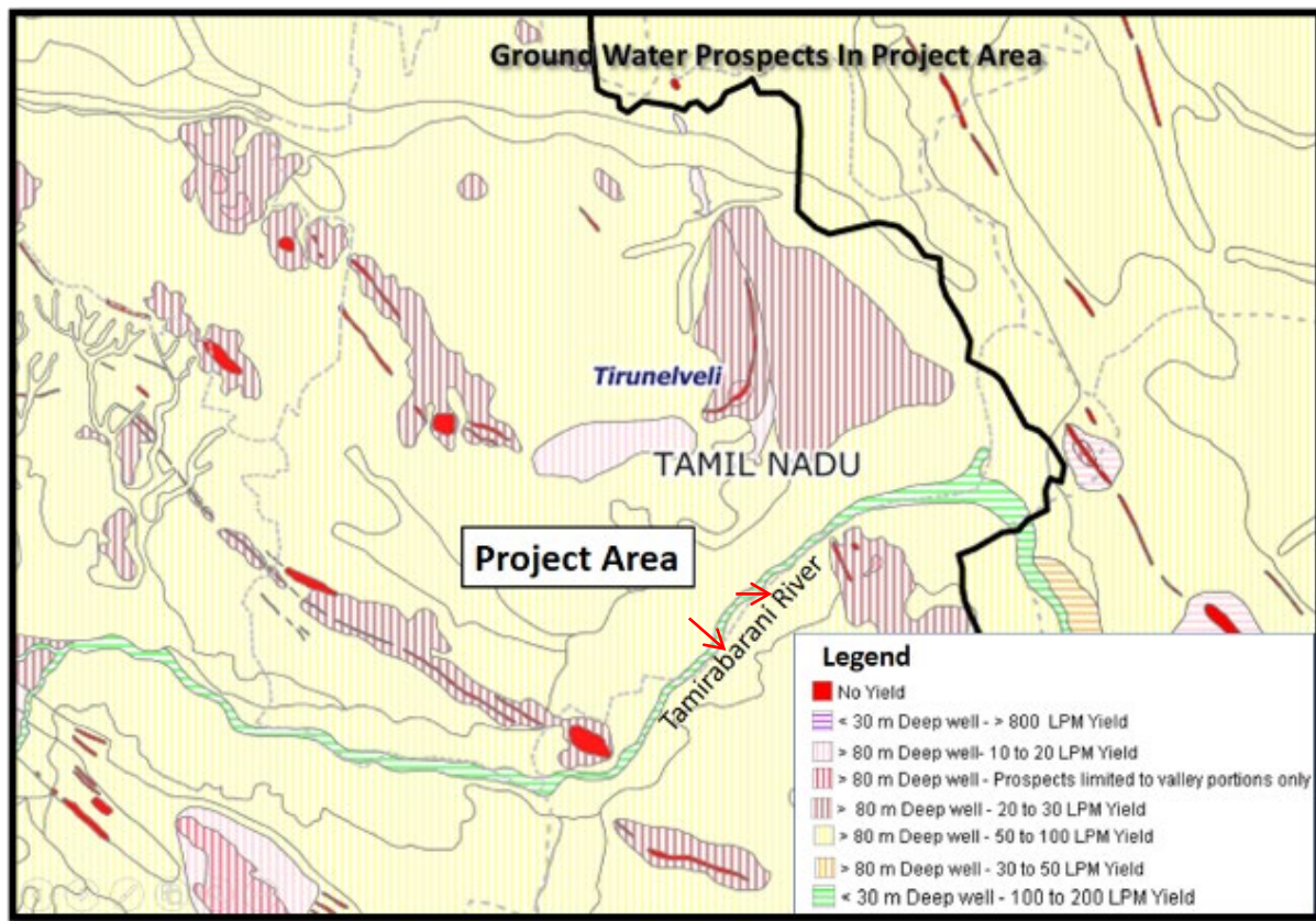
Figure 13: Ground Water Prospects in Project Area
