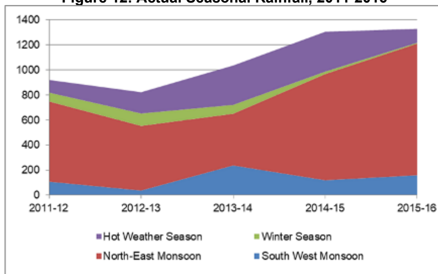
Figure 12: Actual Seasonal Rainfall, 2011-2016
