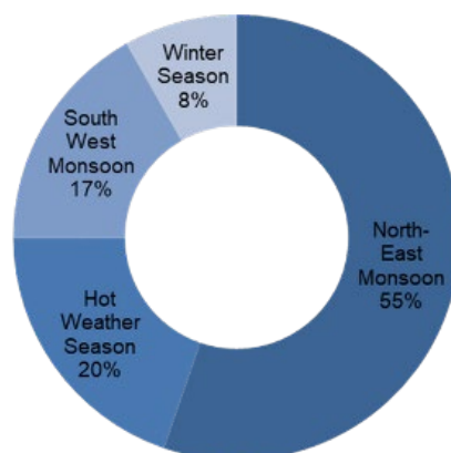
Figure 11: Seasonal Distribution of Normal Annual Rainfall
