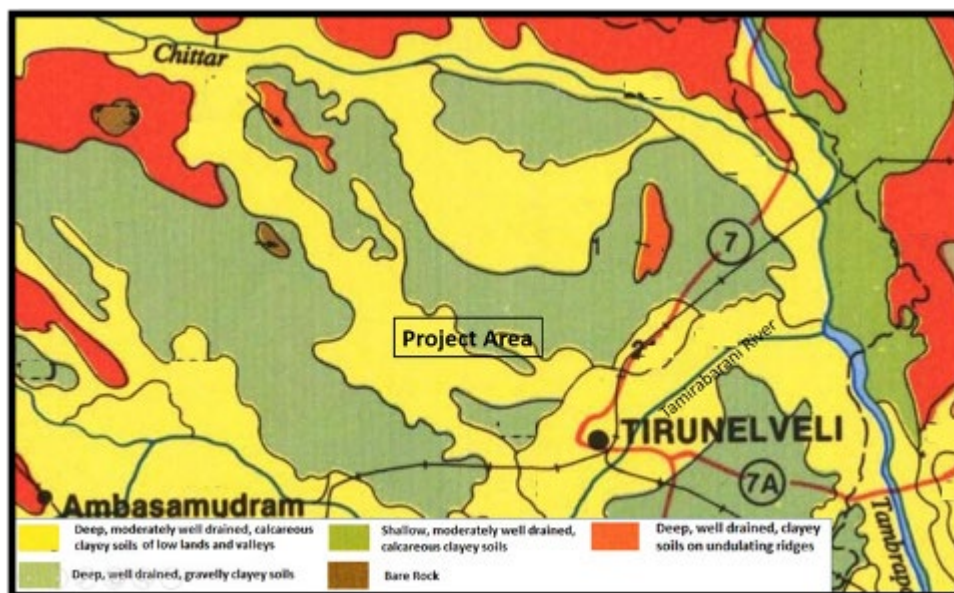
Figure 9: Geomorphology of Project Area
