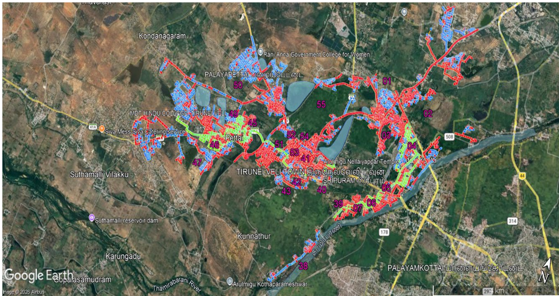
Figure 7: Proposed Sewer Network and Manholes
